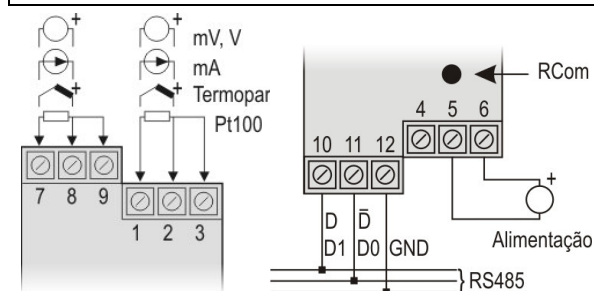
Figure 2 – Electrical Connections
