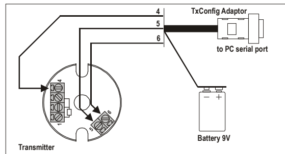
Figure 1 – Adaptor connections to the TxBLOCK
