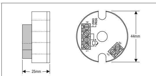
Figure 3 – TxBlock dimensions
