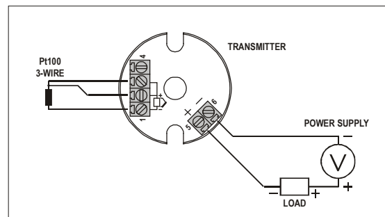
Figure 4 – TxBlock wiring (Pt100)
