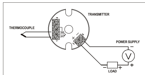
Figure 5 – TxBlock wiring (Thermocouple)
