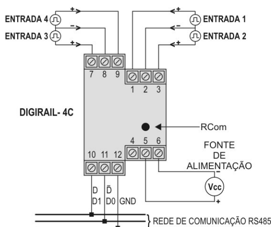
Figure 2 – Electrical Connections
